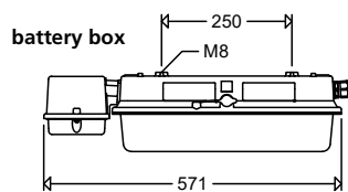
e856F ... H (with battery box)
