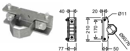
Single mounting: MAU 1 76/170 M10
